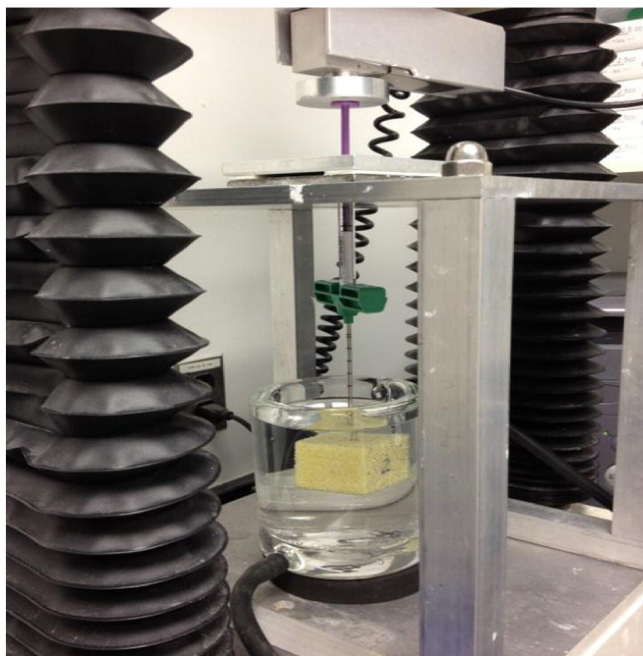
Fig. 2. The mechanical testing setup utilized.
